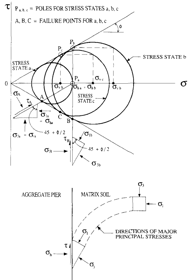
FIG. 4. Theoretical Stress States During Uplift of an Aggregate Pier
